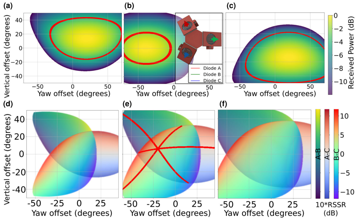
Fig. 8 | Plots characterizing the relative received light power across photodiode pairs in Pisces. Power received at a distance of 0.30 m with different yaw and vertical offsets at (a) Photo Diode (PD) A (-4dB highlighted in red), (b) PD B (-2 dB highlighted in red) and (c) PD C (-6dB highlighted in red). Also shown are the Received Signal Strength Ratio (RSSR) plots for each diode pair AB, AC, and BC with a horizontal LED-receiver distance of (d) 0.15 m, (e) 0.30 m, and (f) 1.50 m.
