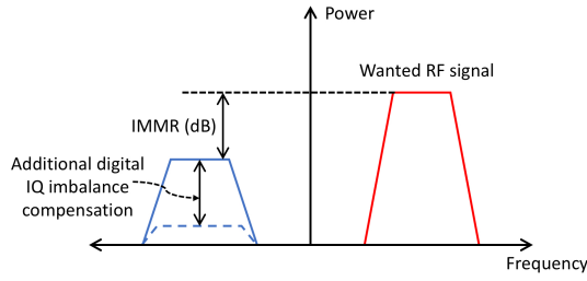
Figure 2: Effect of IQ imbalance quantified through IMRR.
