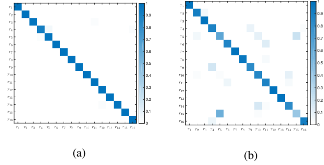
Figure 6: Confusion matrix relative to two experiments with same devices and different locations: (a) overall accuracy is 98.60%; (b) overall accuracy is 87.13%.
